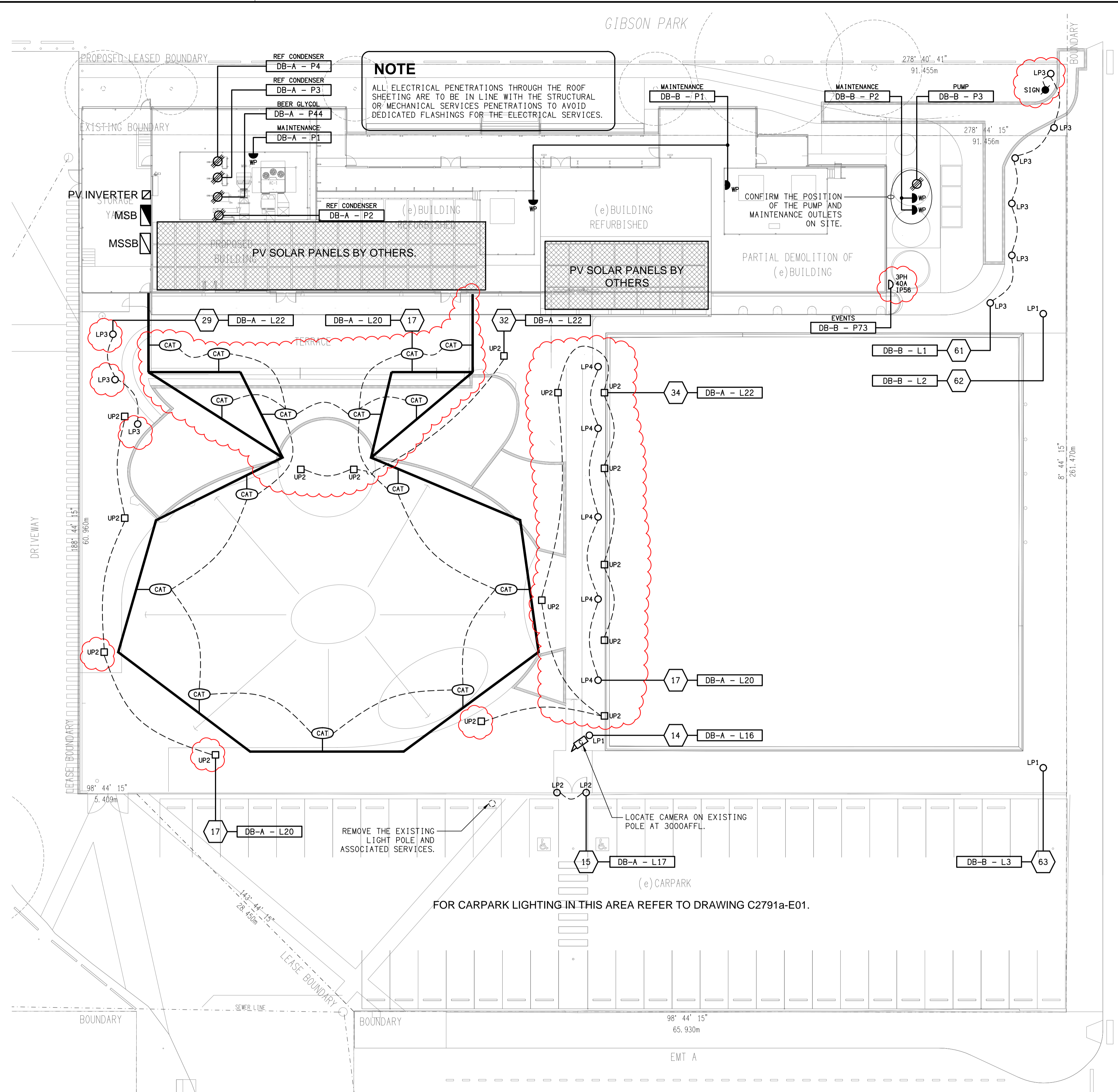
SITE PLAN LANDSCAPE LIGHTING & ROOF SCALE 1:200
